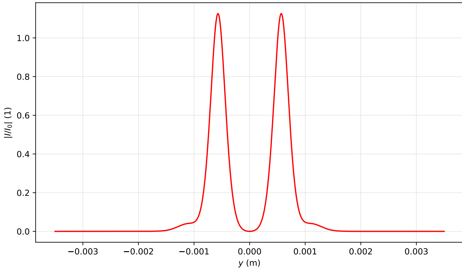
Intensity profile I(x=0, y, z=0.796)/I_0 , P_{in}=6.0P_{cr} , artificial time
